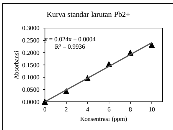
Gambar 3. Kurva standar larutan \text{Pb}^{2+}
