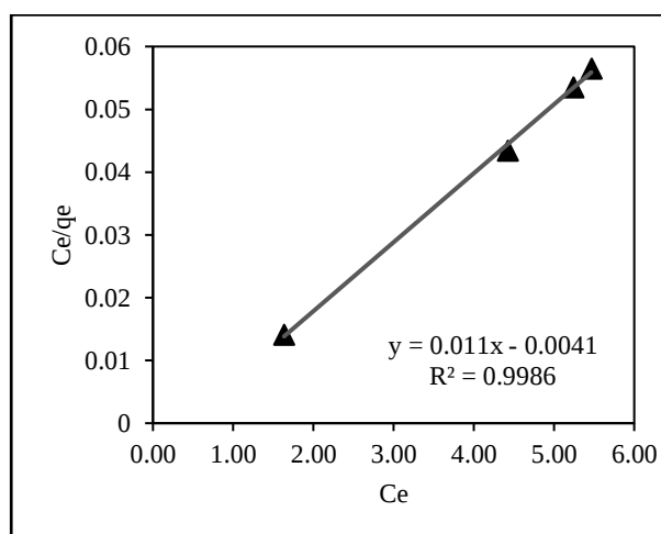
Gambar 8. Grafik adsorpsi isoterm Langmuir
